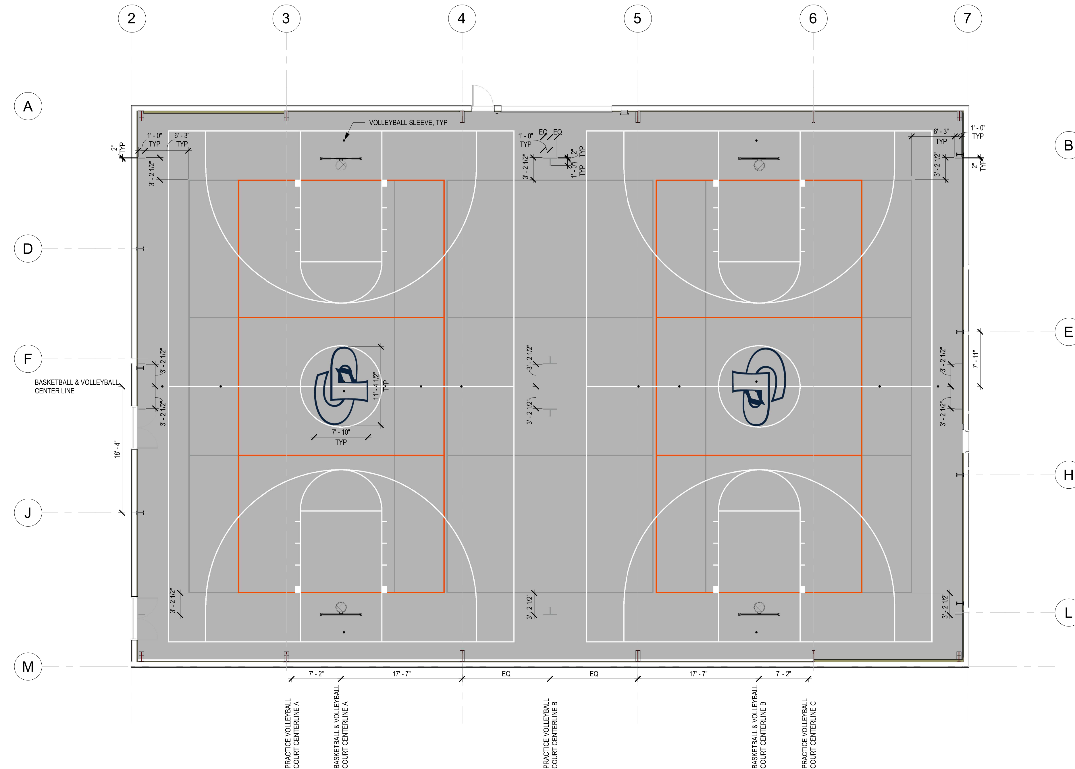
GYM LINE LAYOUT PLAN SCALE: 1/8" = 1'-0"
